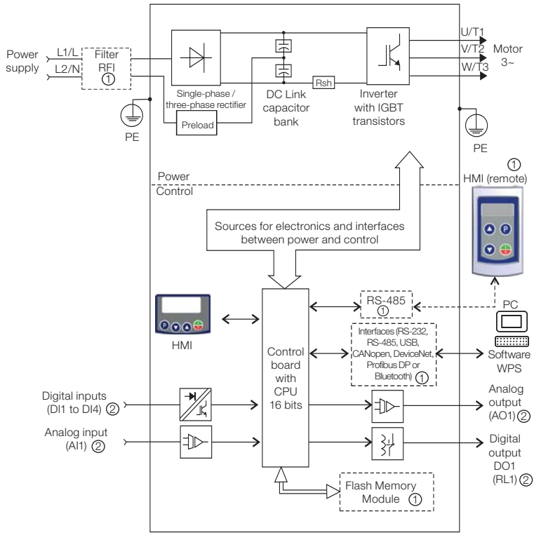
Figure 2.2: Block diagram of CFW300 for frame size A 110 V
