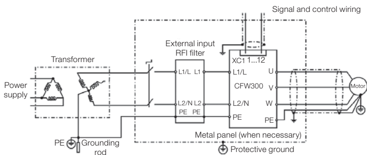
Figure 3.5: Connection of the RFI filter - general conditions
