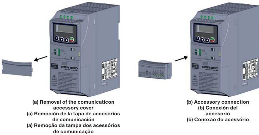
Figure A3: (a) and (b) Slot 1 - Communication accessory or external HMI
