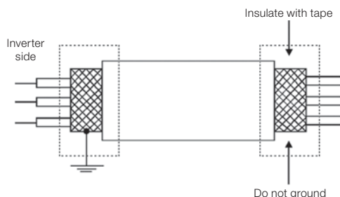
Figure 3.4: Shield connection
