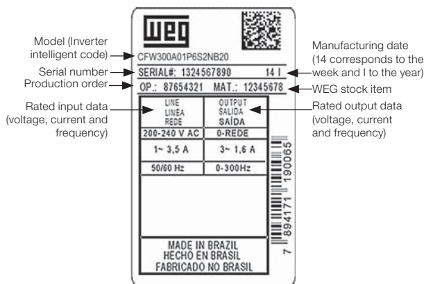
CFW300 Side Label
