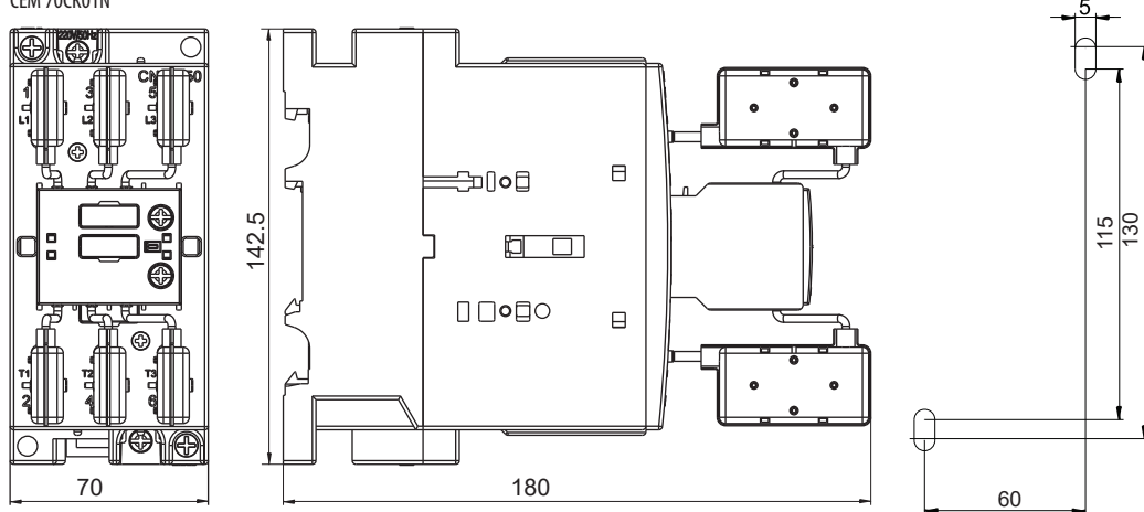
CEM 70CK01N
