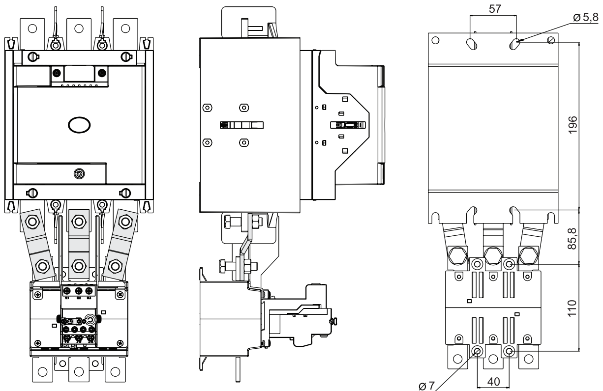
CEM450E/560E + RE317D (200...420A)
