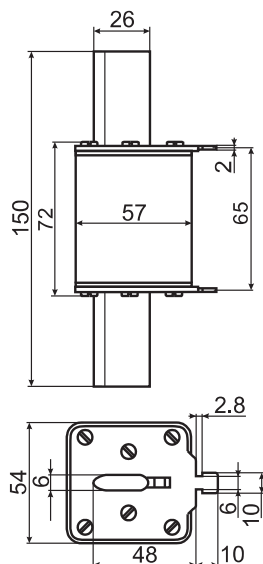
NV/NH 2
