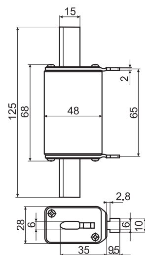
NV/NH 0
