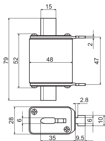
NV/NH 00
