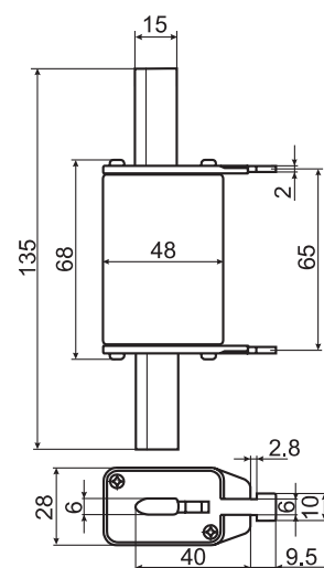
NV/NH 1 C
